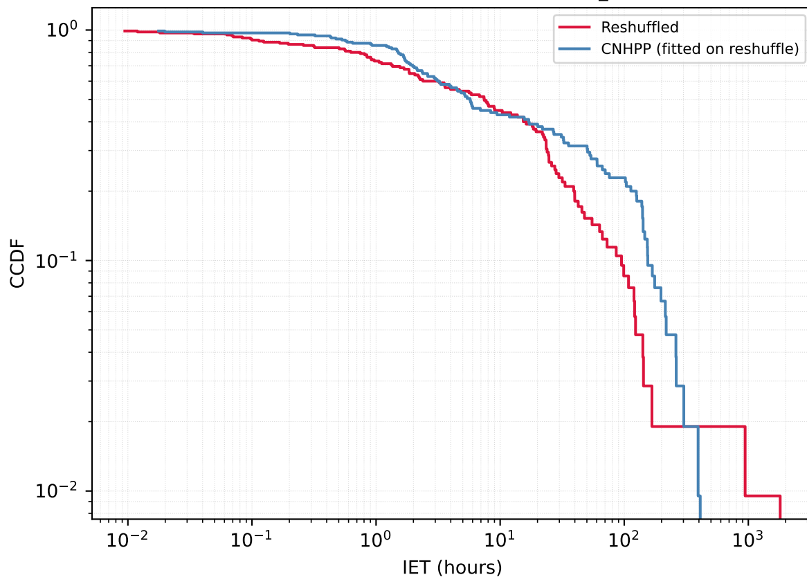
User 1551829597 - Reshuffled vs CNHPP A_{\text{fit}}=0.8787
